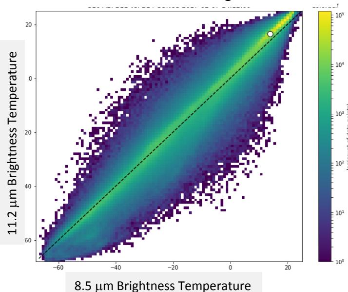
8.5 \mu\text{m} vs. 11.2 \mu\text{m} Brightness Temperature for one CONUS scene using ABI data
