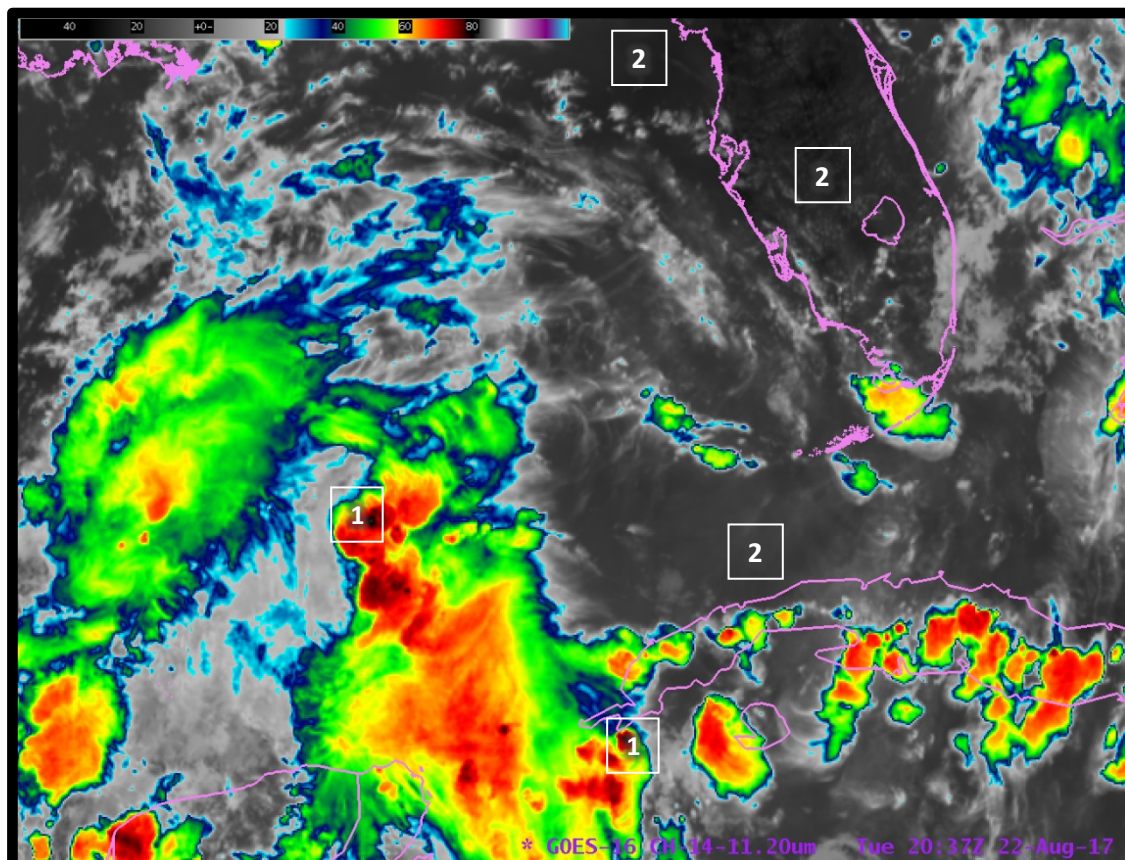
GOES-16 11.2 \mu\text{m} Infrared Imagery, 2027 UTC on 22 August 2017 showing a tropical wave over the southeastern Gulf of Mexico
